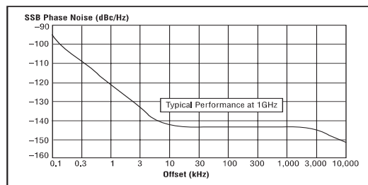
Typical phase noise performance at 1 GHz
